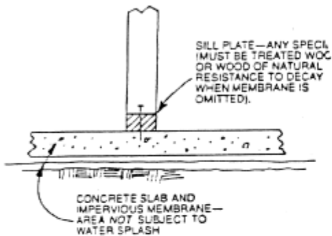
UNDER-FLOOR CLEARANCE
