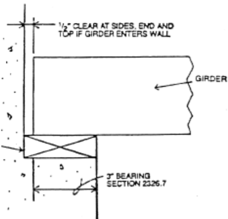
PROTECTION AGAINST DECAY GIRDERS
