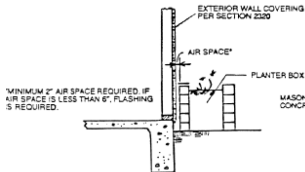
PROTECTION AGAINST DECAY PLANTER BOXES
