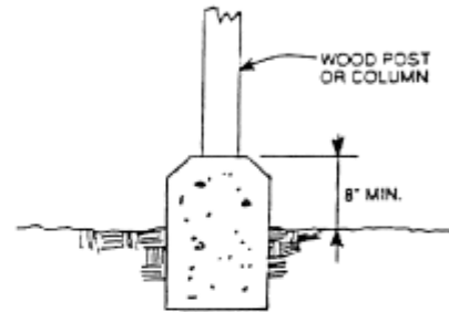
PROTECTION AGAINST DECAY COLUMNS AND POSTS
