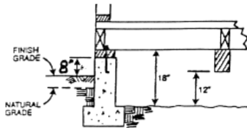
UNDER-FLOOR CLEARANCE
